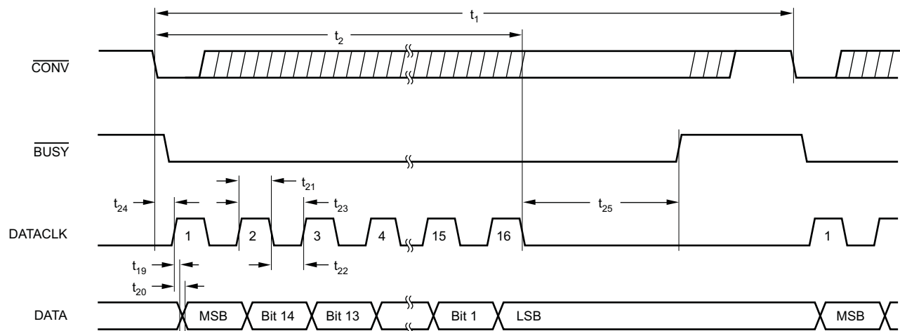
Figure 41. Serial Data Timing, External Clock, Clocking During the Next Conversion (EXT/INT High, CS Low)
