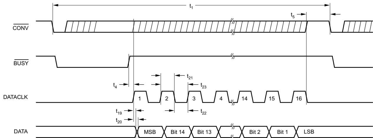
Figure 40. Serial Data Timing, External Clock, Clocking After the Conversion Completes (EXT/INT High, CS Low)
