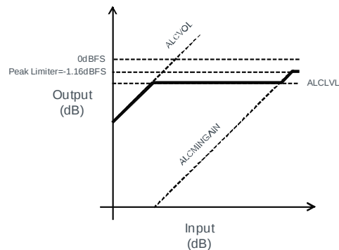
Figure 30. ALC Level diagram
