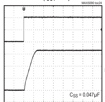
STARTUP WAVEFORM ( I_{OUT} = 2A )
