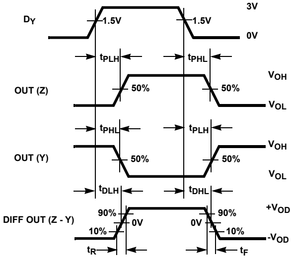
SKEW = |t_{PLH}(Y \text{ or } Z) - t_{PHL}(Z \text{ or } Y)| FIGURE 2B. MEASUREMENT POINTS
