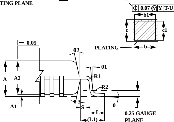
DETAIL F
