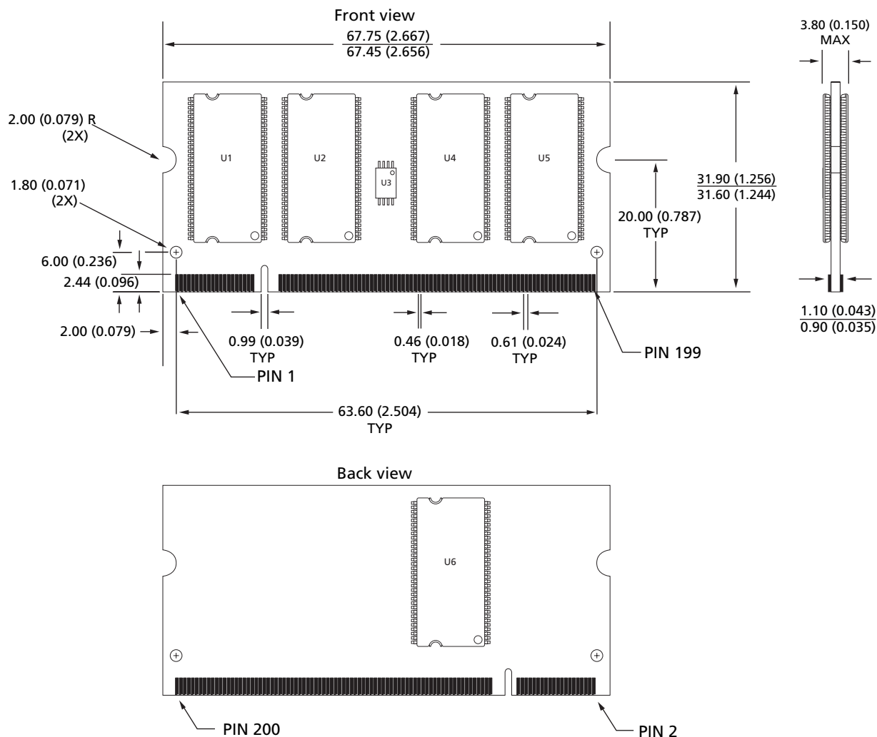
Figure 3: 200-Pin SODIMM Dimensions
