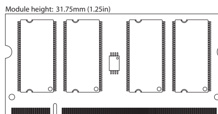
Figure 1: 200-Pin SODIMM (MO-224 R/C C)
