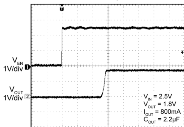
Enable Turn-On Delay and Rise Time
