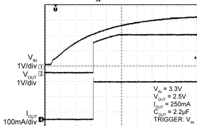
V IN Soft Turn-On
