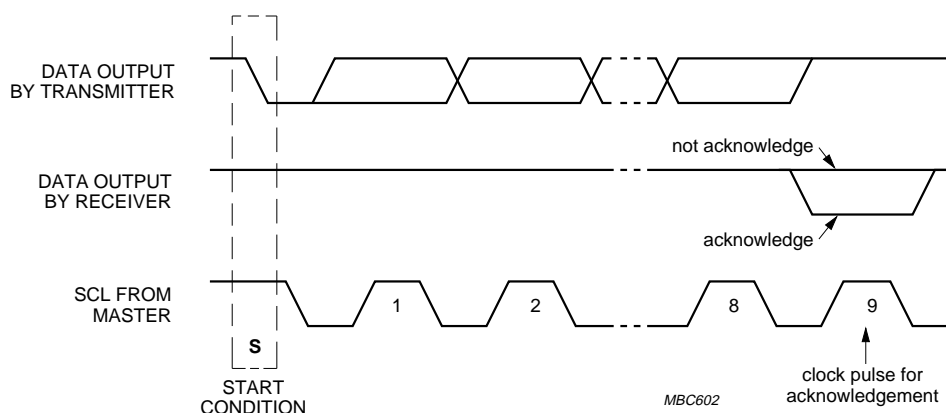
Fig.6 Acknowledgment on the I 2 C-bus.
