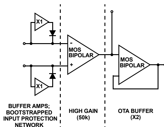
FIGURE 1. FUNCTIONAL DIAGRAM
