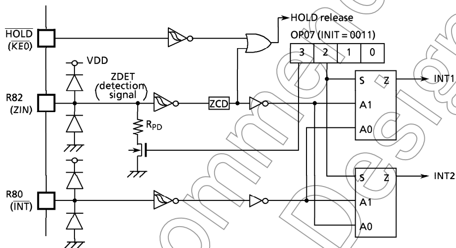
Figure 3-19. Zero-cross Detector
