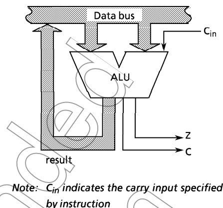
Figure 2-11. ALU
