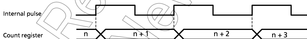
Figure 3-11. Timer Mode Timing chart
