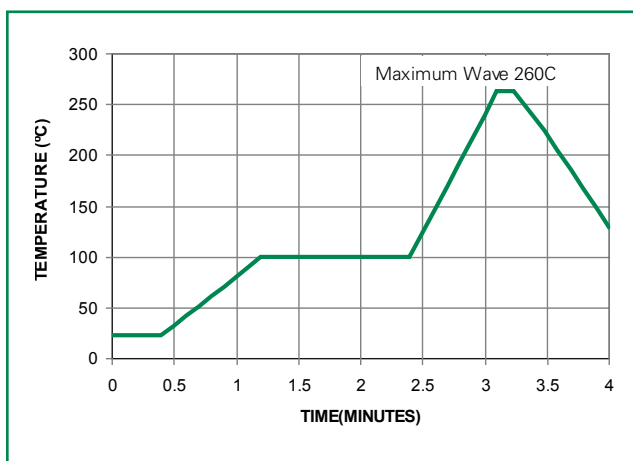
Figure 2 - Lead-free Profile
