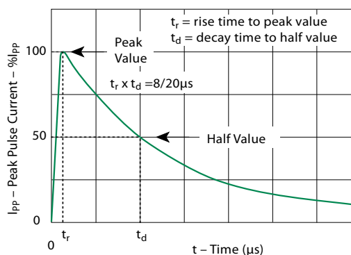
Figure 6 - Pulse Waveform
