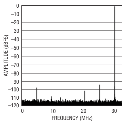
LTC2162: 64k Point FFT, f_{IN} = 30\text{MHz} , -1dBFS, 65Msps
