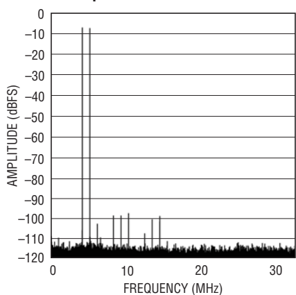
LTC2162: 64k Point 2-Tone FFT, f_{IN} = 69\text{MHz} , 70\text{MHz} , -7dBFS, 65Msps
