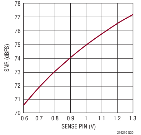
LTC2161: SNR vs SENSE, f_{IN} = 5\text{MHz} , -1dBFS
