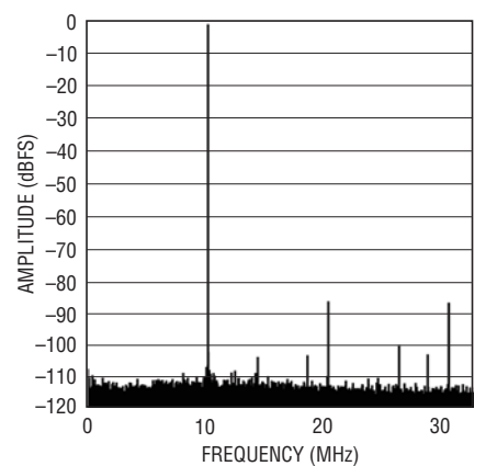
LTC2162: 64k Point FFT, f_{IN} = 140\text{MHz} , -1dBFS, 65Msps
