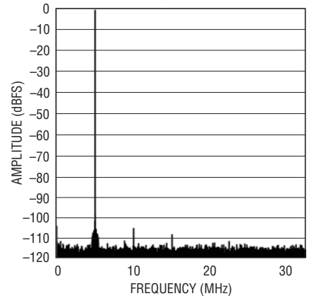
LTC2162: 64k Point FFT, f_{IN} = 5\text{MHz} , -1dBFS, 65Msps
