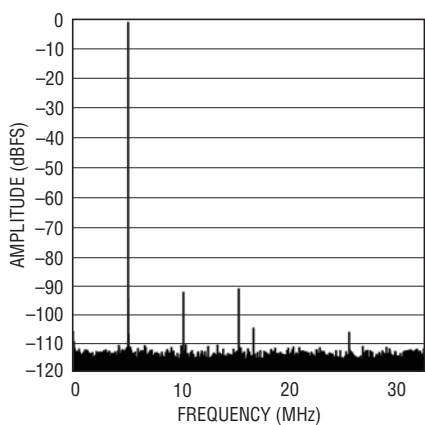
LTC2162: 64k Point FFT, f_{IN} = 70\text{MHz} , -1dBFS, 65Msps
