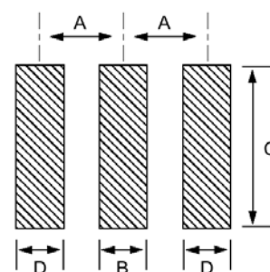
Figure 2) Land Pattern
