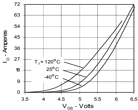
Fig. 7. Input Admittance
