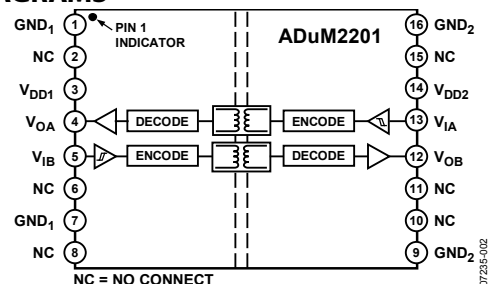
Figure 2. ADuM2201
