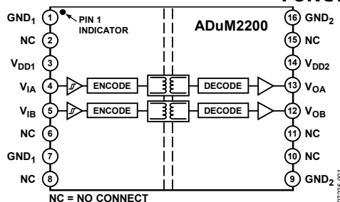
Figure 1. ADuM2200
