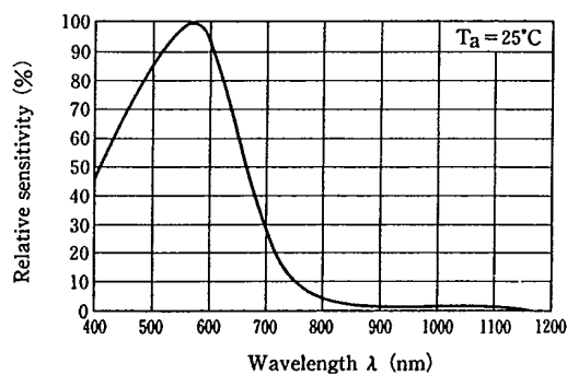
Fig. 4 Spectral Sensitivity
