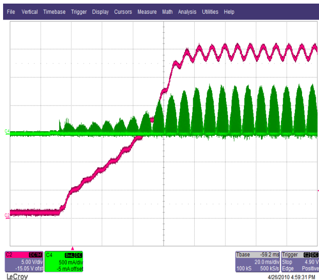
Figure 23 – 90 VAC, Full Load. Upper: I_{DRAIN} , 0.5 A / div. Lower: V_{OUTPUT} , 5 V, 20 ms / div.
