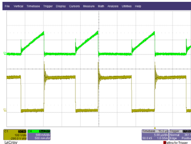
Figure 19 – 90 VAC, Full Load. Upper: I_{DRAIN} , 0.5 A / div. Lower: V_{DRAIN} , 100 V, 5 \mu s / div.
