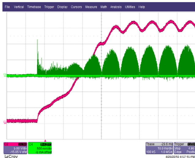
Figure 24 – 265 VAC, Full Load. Upper: I_{RIPPLE} , 0.5 A / div. Lower: V_{OUTPUT} , 5 V, 10 ms / div.
