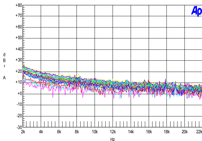
Figure 41 – 2 kHz – 22 kHz.
