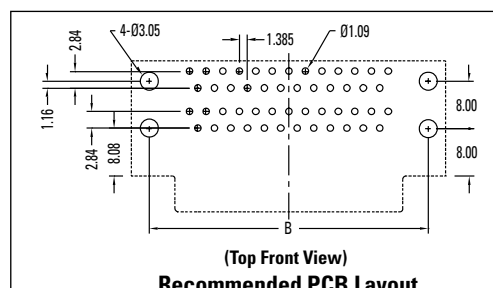
(Top Front View) Recommended PCB Layout
