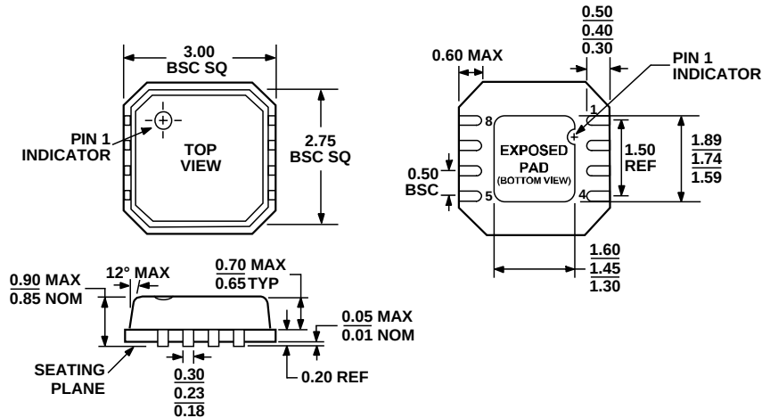
Figure 52. 8-Lead Lead Frame Chip Scale Package [LFCSP_VD] 3 mm x 3 mm Body, Very Thin, Dual Lead (CP-8-2)
