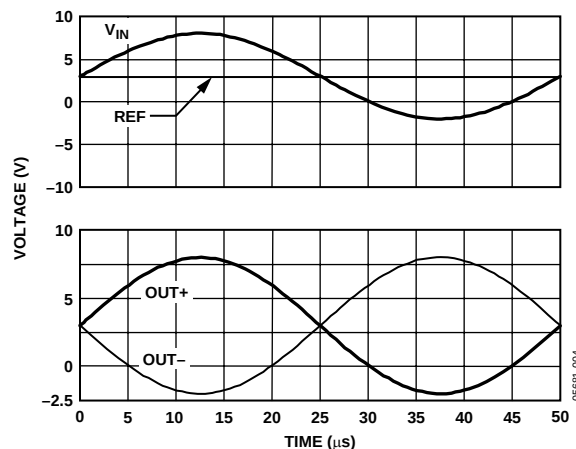
Figure 43. Typical Input/Output Response—Equal Input/Reference
