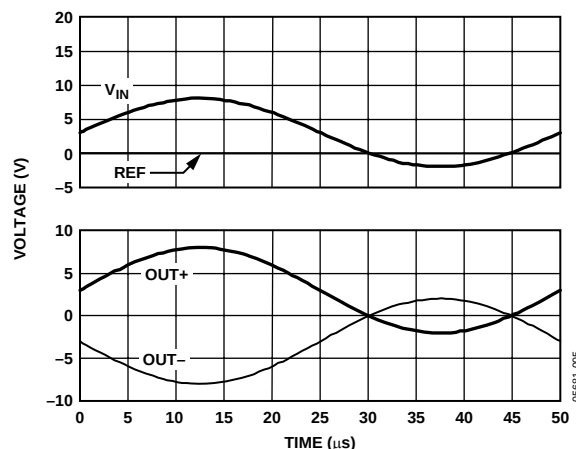
Figure 44. Typical Input/Output Response—Unequal Input/Reference
