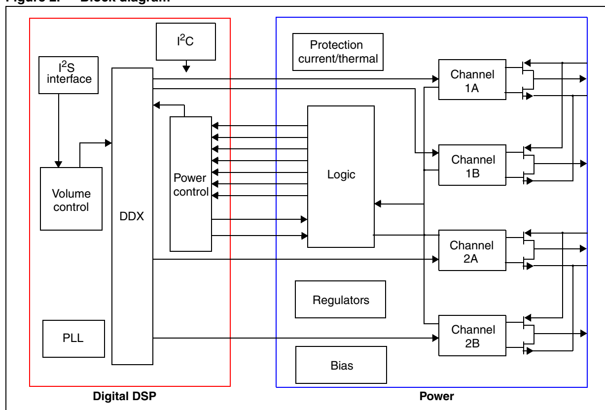
Figure 2. Block diagram
