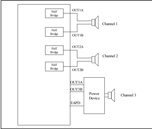
Figure 11. OCFG = 10
