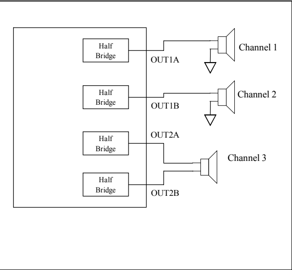
Figure 10. OCFG = 01
