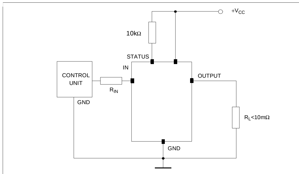
Fig. 1: Peak Short Test Circuit
