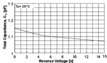
Figure 6. Total Capacitance
