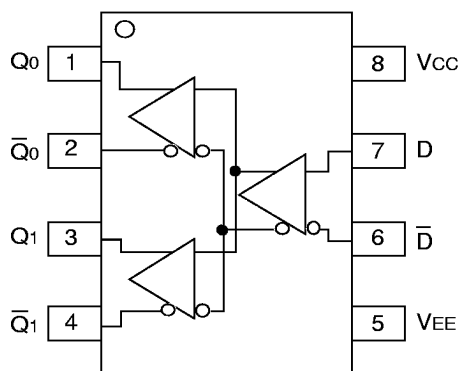
SOIC TOP VIEW
