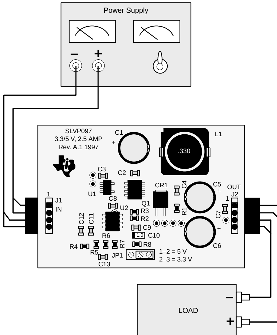
Figure 1–3. I/O Connections
