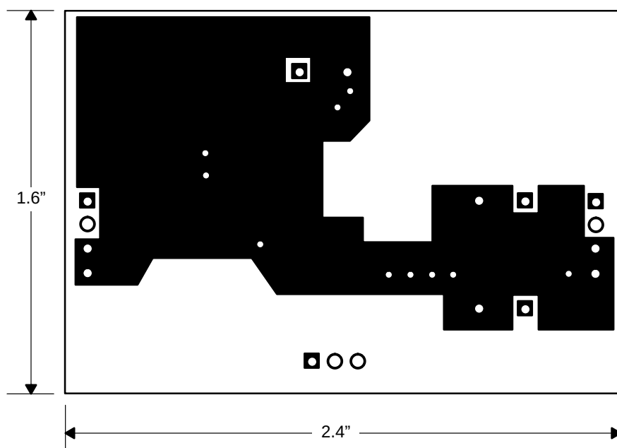
Figure 1–6. Bottom Layer
