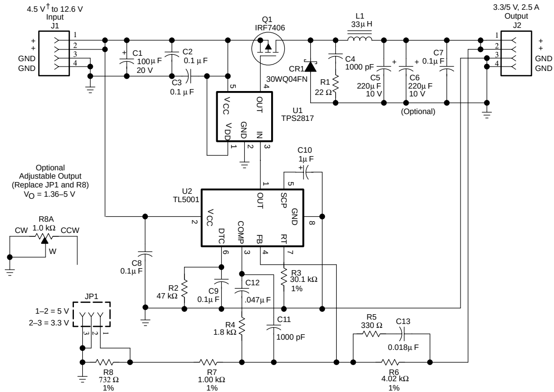
Figure 1–2. SLVP097 Schematic
