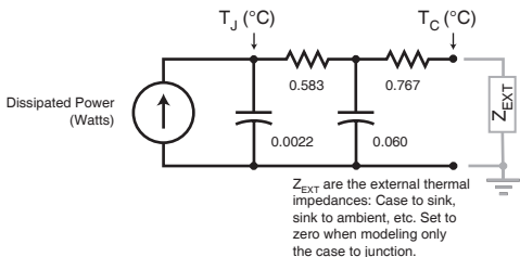
FIGURE 24b. TRANSIENT THERMAL IMPEDANCE MODEL
