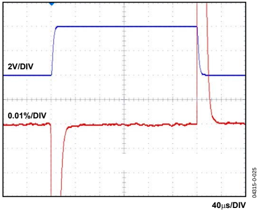
Figure 11. Settling Time
