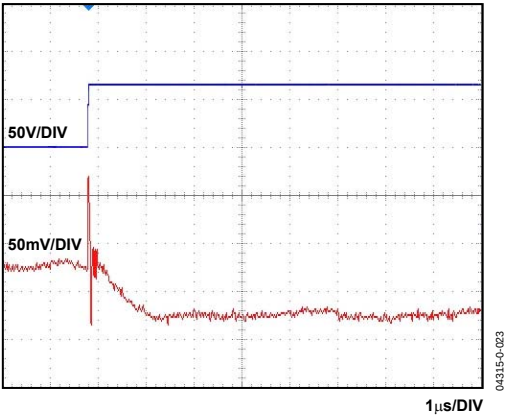
Figure 12. Common-Mode Response
