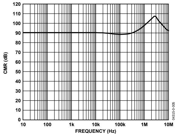
Figure 5. CMR vs. Frequency
