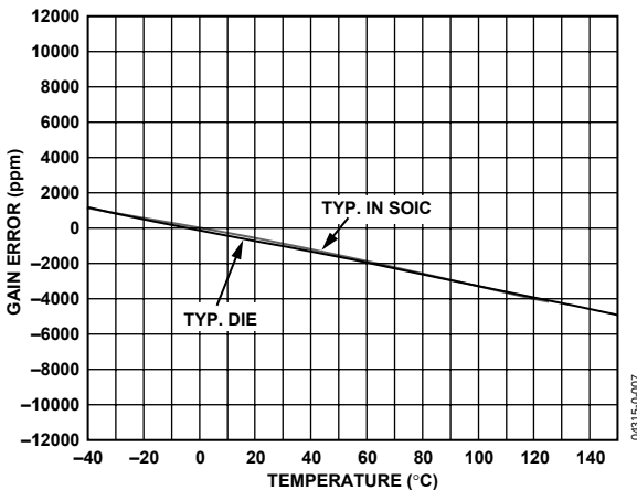
Figure 6. Gain Drift
