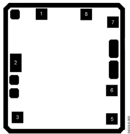
Figure 2. Metallization Diagram
