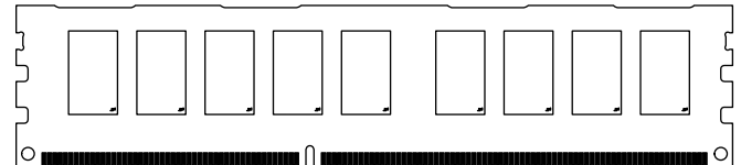
Figure 1: 240-Pin UDIMM (MO-269 R/C E)
