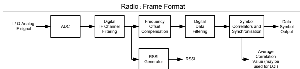
Figure 38: Demodulator Simplified Block Diagram
