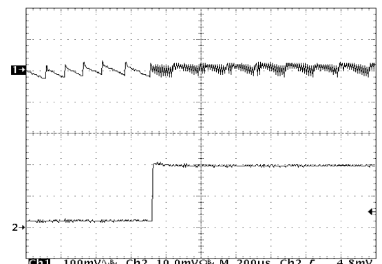
Figure 24. Load Transient Response for V_{IN} = 1.8 V
