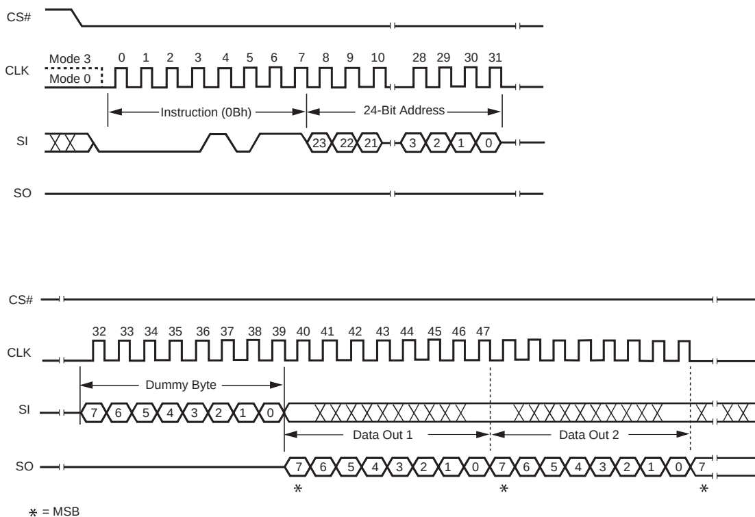
Figure 7.7 Fast Read Instruction Sequence Diagram
