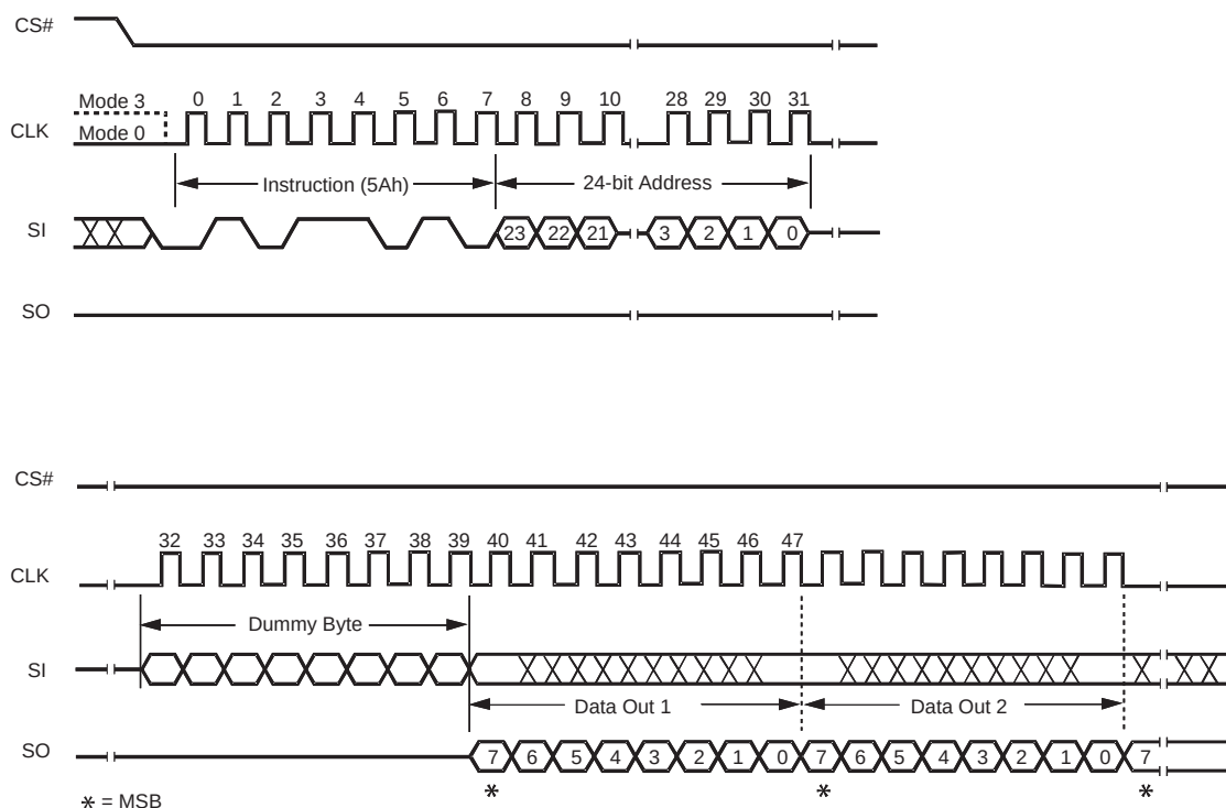
Figure 7.36 Read SFDP Register Instruction Sequence Diagram
