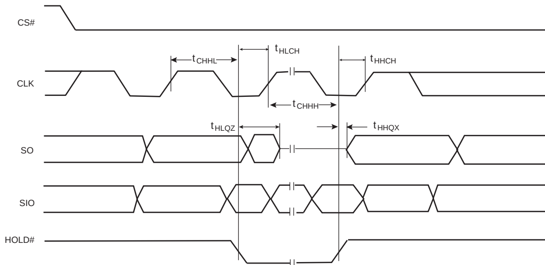
Figure 8.5 Hold Timing
