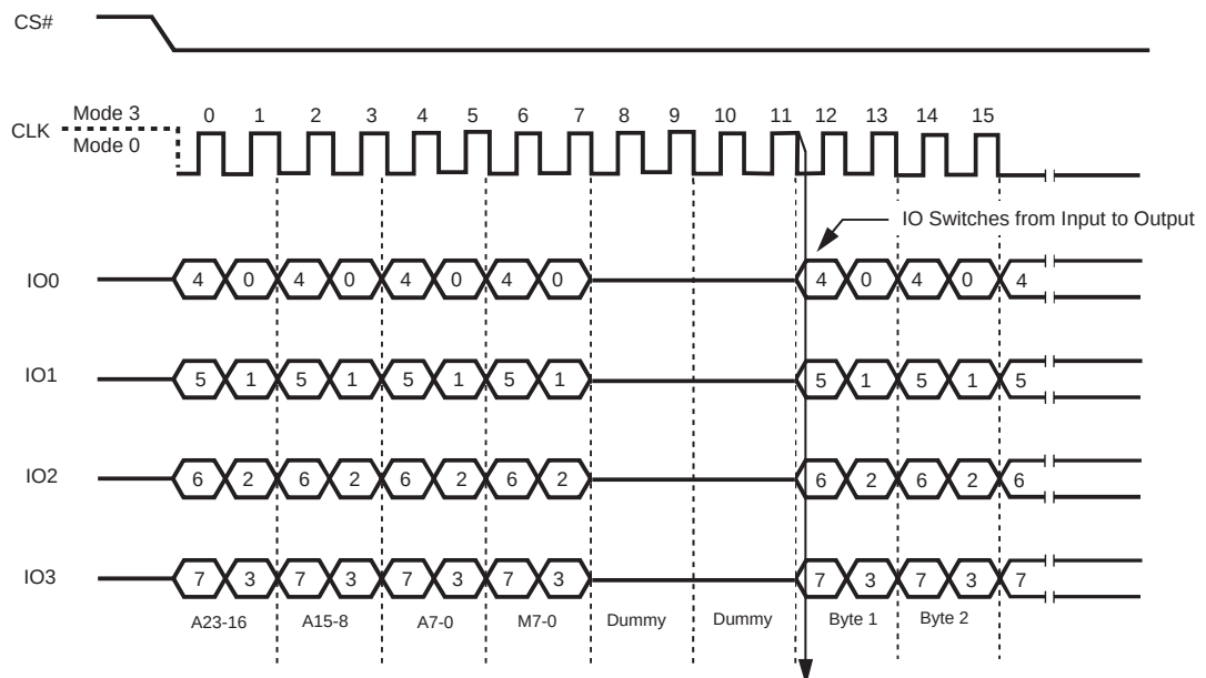
Figure 7.13 Fast Read Quad I/O Instruction Sequence (Previous instruction set M5-4 = 10)
