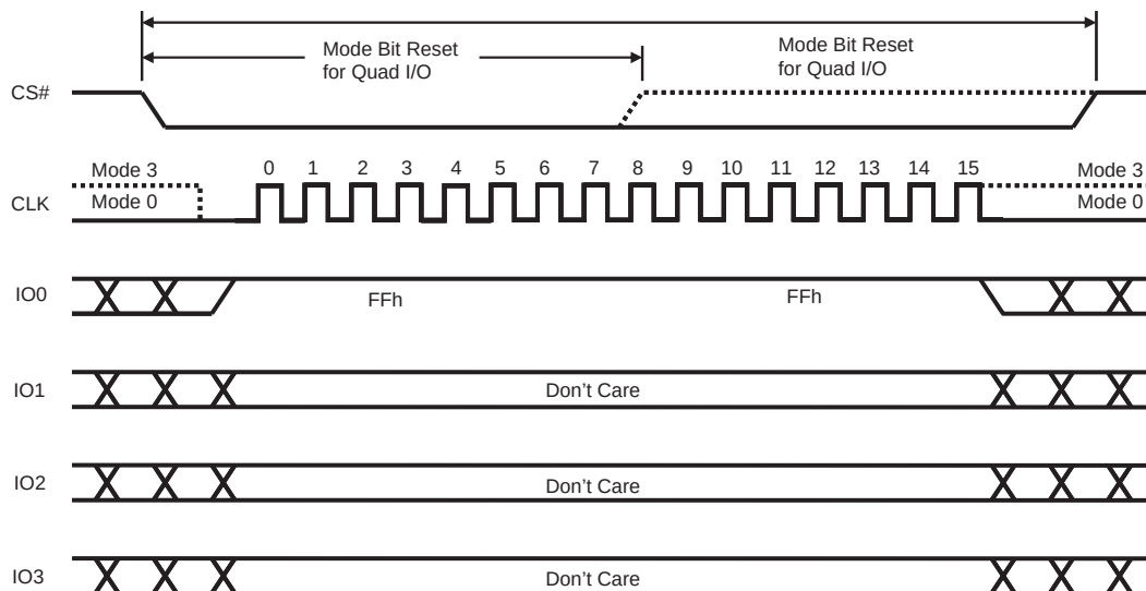
Figure 7.19 Continuous Read Mode Reset for Fast Read Dual/Quad I/O
