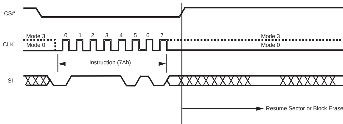
Figure 7.27 Erase/Program Resume Instruction Sequence
