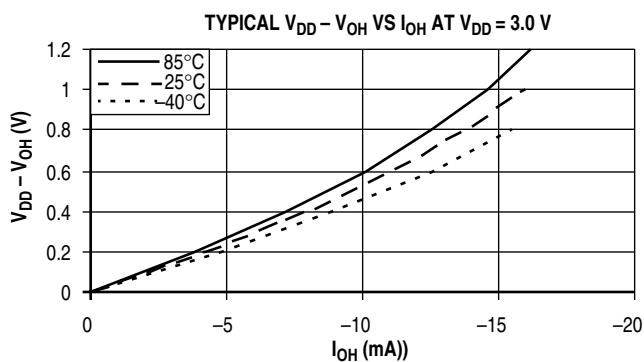
Figure A-4. Typical High-Side (Source) Characteristics — Low Drive ( PTxDSn = 0 )
