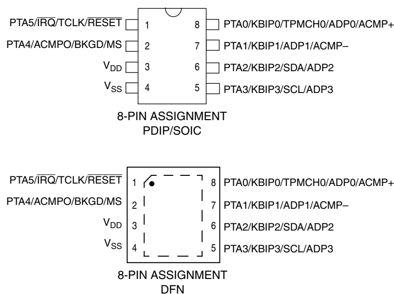
Figure 2-1. 8-Pin Packages
