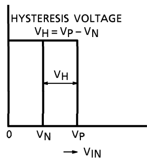
● TRANSFER CHARACTERISTICS
