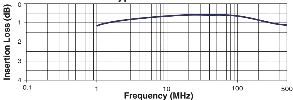
CX2078 - Typical Insertion Loss
