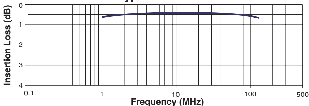
CX2081 - Typical Insertion Loss
