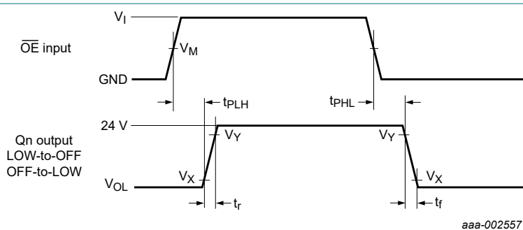
Fig. 10. The output enable ( \overline{OE} ) input to data output (Qn) propagation delays and (Qn) output rise and fall times
