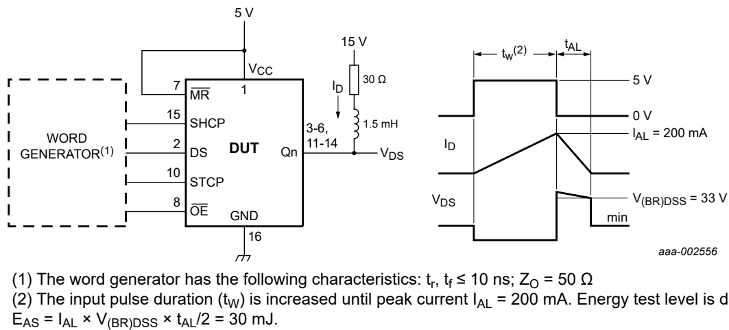
Fig. 9. Test circuit and waveform for measuring single-pulse avalanche energy
