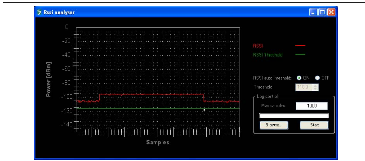
Figure 31: RSSI Analyzer Window
