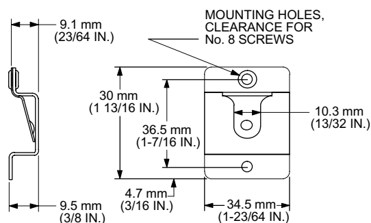
MOUNTING BRACKET
