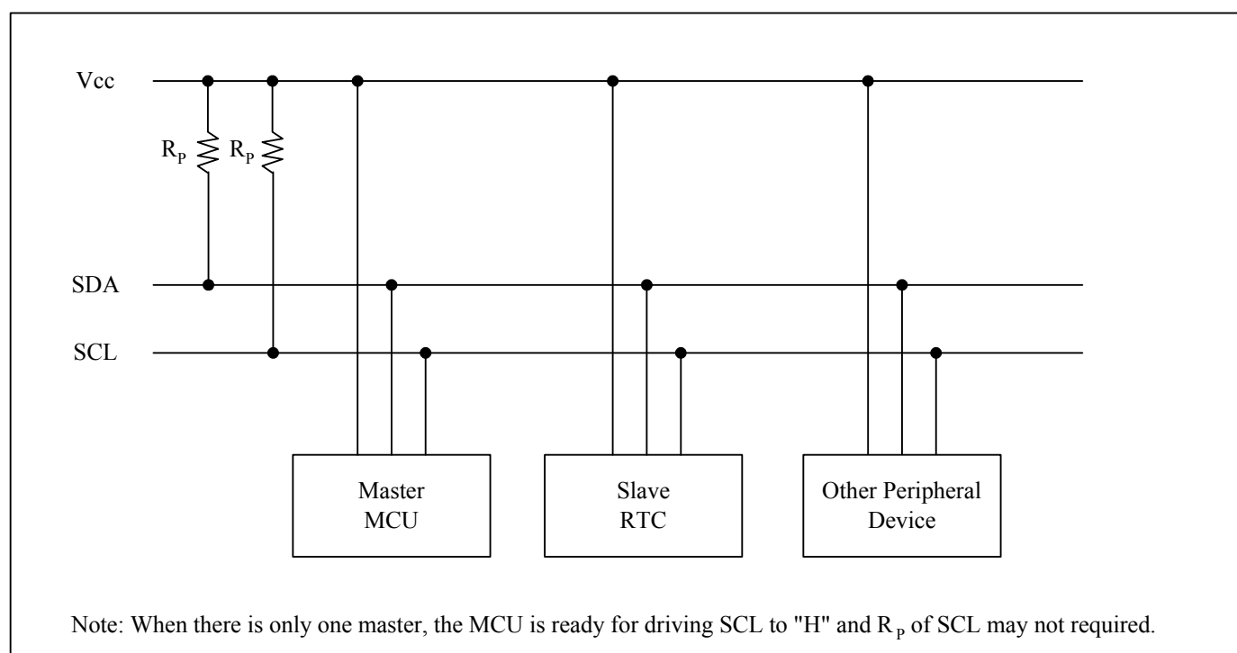
Fig 1. System configuration
