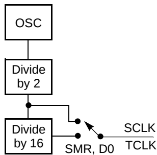
Figure 48. SCLK Circuit
