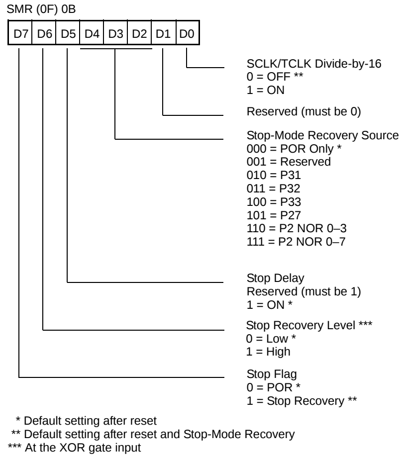
Figure 47. Stop-Mode Recovery Register
