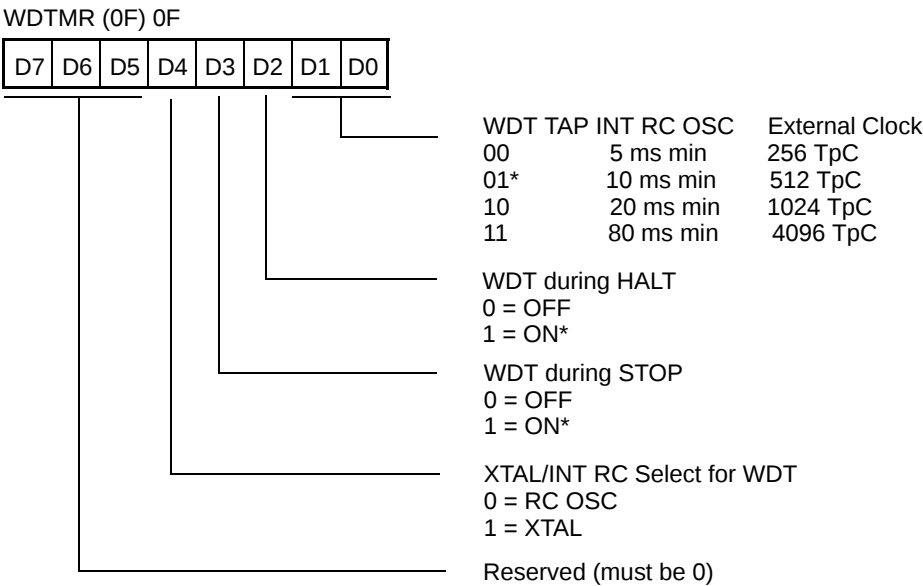
Figure 19. Watch-Dog Timer Register—(0F) 0FH: Write Only
