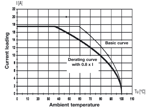
TOP 1.5GS/90 2STI OR with Conductor H07V-K1.5 mm 2
