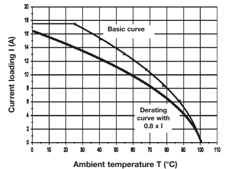
LMZF 5.08/180/24 poles with Conductor H07V-K1.5 mm 2
