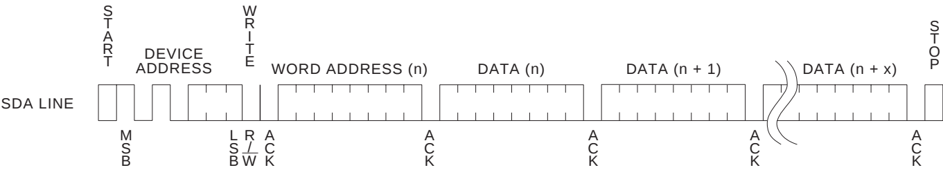
Figure 3. Page Write
