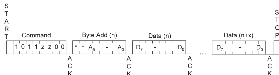
Figure 9-2. Write EEPROM
