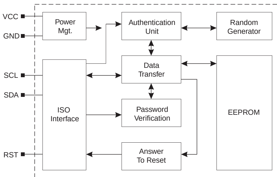
Figure 2-1. Block Diagram
