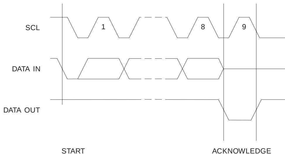
Figure 10-3. Output Acknowledge
