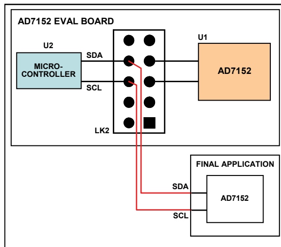
Figure 7. AD7152 Evaluation Board as USB-to-I 2 C interface
