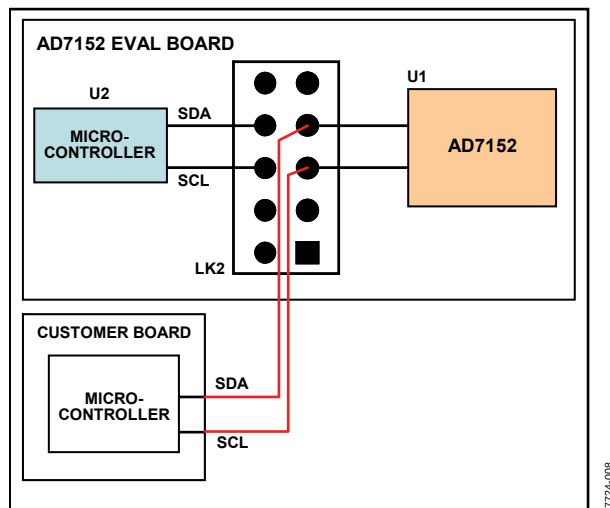
Figure 8. AD7152 Evaluation Board Software Development Platform
