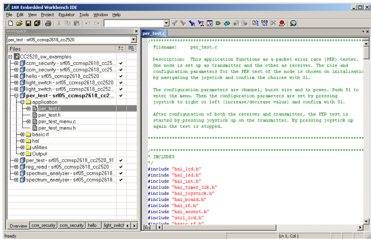
Figure 2 IAR EW
