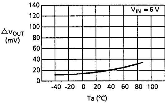
1.14 Load stability ( V_{OUT} ) – Temperature
