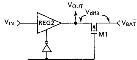
Figure 6 Definitions of V_{dif3}
