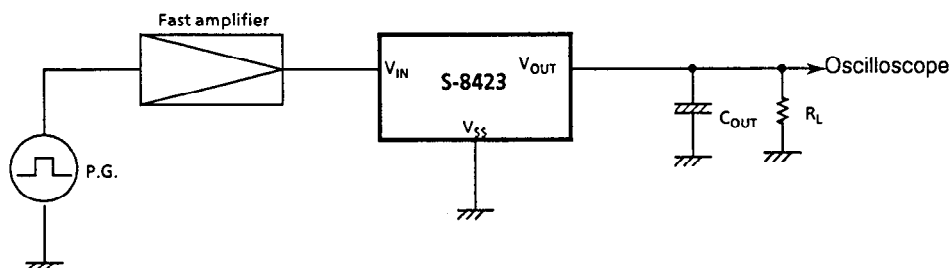
Figure 9 Measuring circuit
