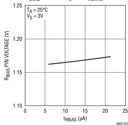
R_{\text{BIAS}} Pin Voltage vs I_{\text{RBIAS}}
