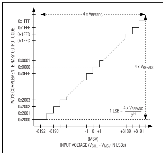
Figure 7. ±5V Bipolar Transfer Function
