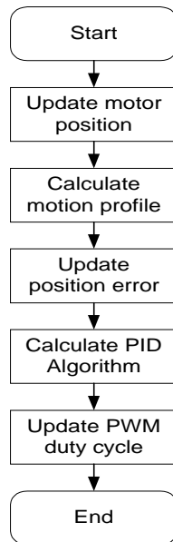
Fig. 6 ISR flowchart
