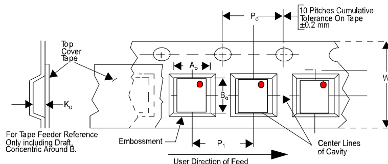
Figure 15. Tape and Reel Mechanical Data
