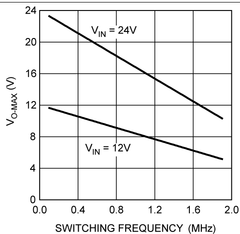
Figure 13. V_O-MAX vs f_SW, LM3402 (T_A = 25°C)
