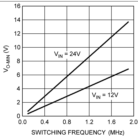
Figure 14. V_O-MIN vs f_SW, LM3402 (T_A = 25°C)
