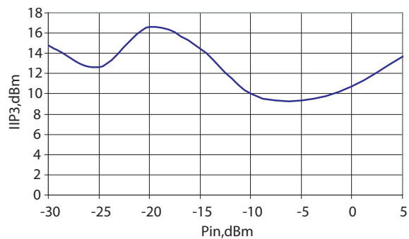
Figure 17. Bypass Mode IIP3 vs Input Power
